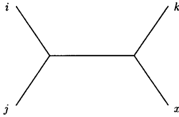
FIG. 1. A phylogenetic X -tree for X = \{i, j, k, x\} .
