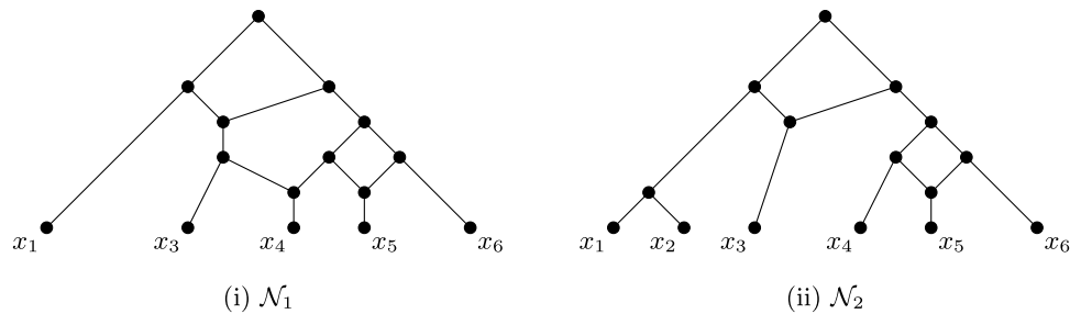
Fig. 2. \mathcal{N}_1 has been obtained from \mathcal{N} in Fig. 1 by reducing x_2 , while \mathcal{N}_2 has been obtained from \mathcal{N} by cutting \{x_3, x_4\} .
