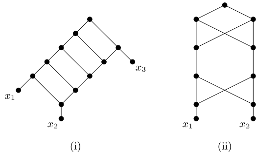
Fig. 3. (i) An orchard network and (ii) a non-orchard network.
