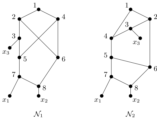
Fig. 5. Two orchard networks \mathcal{N}_1 and \mathcal{N}_2 with \Gamma_{\mathcal{N}_1} = \Gamma_{\mathcal{N}_2} , but \Sigma_{\mathcal{N}_1} \neq \Sigma_{\mathcal{N}_2} .
