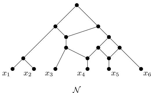
Fig. 1. A phylogenetic network \mathcal{N} on \{x_1, x_2, \dots, x_6\} . Here, \{x_1, x_2\} is a cherry and \{x_3, x_4\} is a reticulated cherry with x_4 the reticulation leaf.
