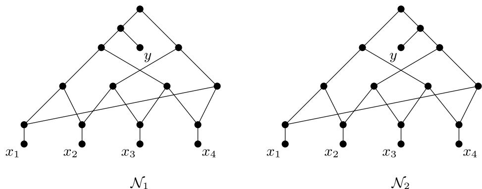
Fig. 4. Two non-isomorphic phylogenetic networks \mathcal{N}_1 and \mathcal{N}_2 , but \Sigma_{\mathcal{N}_1} = \Sigma_{\mathcal{N}_2} .
