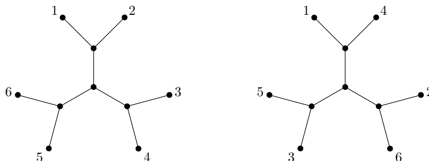
FIGURE 3. Two free ternary X -trees with X = \{1, 2, \dots, 6\} .
