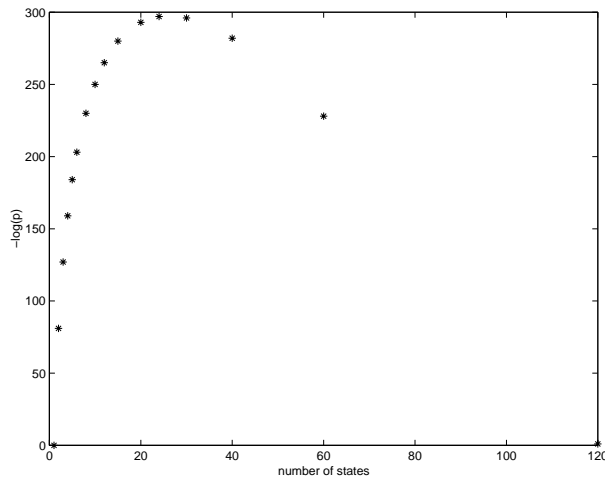
FIGURE 2. Distribution of trivalent phylogenetic trees on 120 leaves by the number of characters states.
