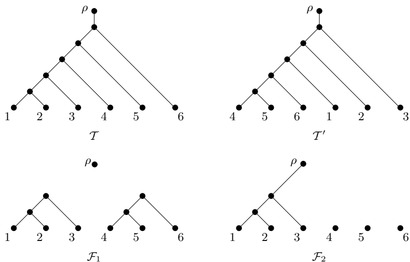
FIGURE 2. \mathcal{F}_1 and \mathcal{F}_2 are agreement forests for \mathcal{T} and \mathcal{T}' .
