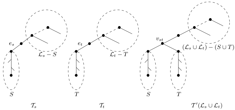
FIGURE 5. The layout of a pair of overlapping components \mathcal{T}_s and \mathcal{T}_t . The set S (resp. T ) is the subset of \mathcal{L}_s (resp. \mathcal{L}_t ) whose members lie below v_{st} in \mathcal{T}' .
