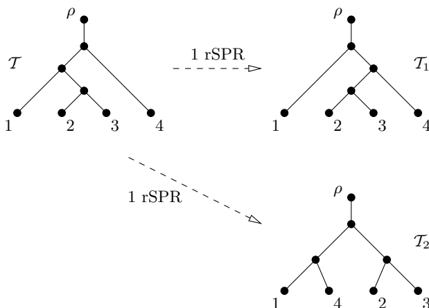
FIGURE 1. Each of \mathcal{T}_1 and \mathcal{T}_2 are obtained from \mathcal{T} by a single rSPR operation.
