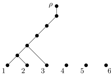
FIGURE 3. A forest of \mathcal{T} that yields an agreement forest for \mathcal{T} and \mathcal{T}' .
