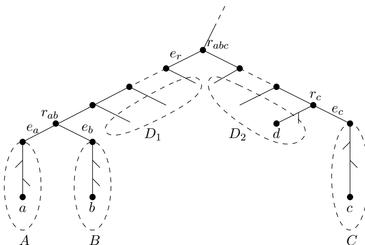
FIGURE 4. The layout of a minimal incompatible triple.
