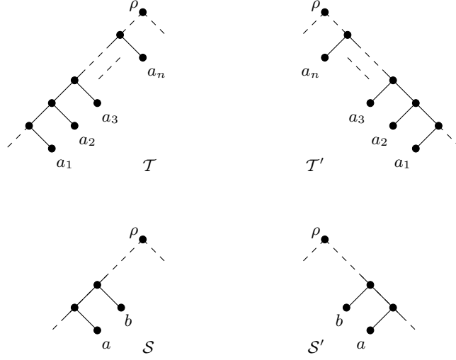
FIGURE 5. Two weighted phylogenetic trees reduced under Rule 2, where \mathcal{S} and \mathcal{S}' are the resulting trees.
