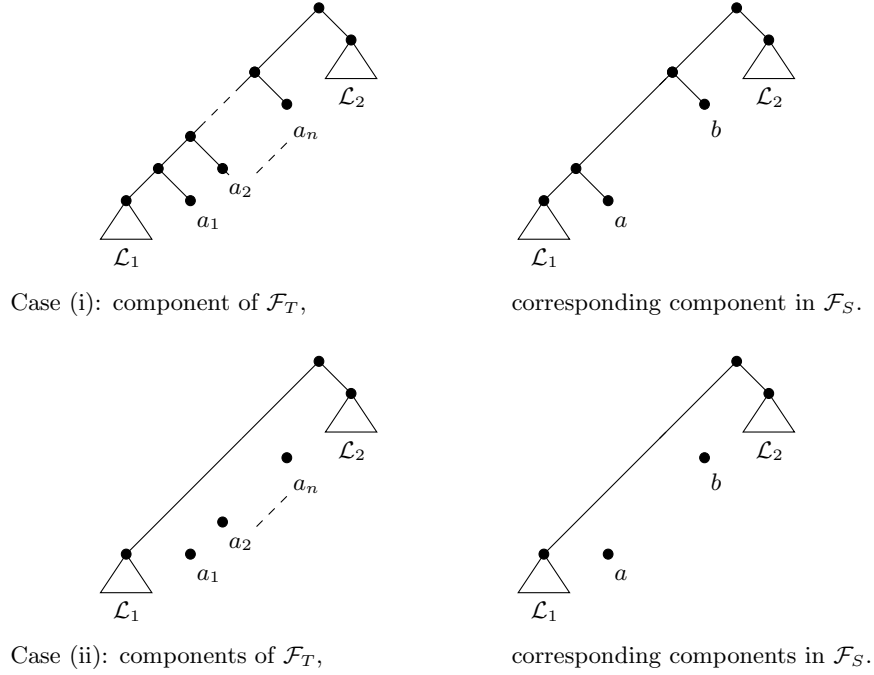
FIGURE 8. Corresponding components of \mathcal{F}_T and \mathcal{F}_S for Cases (i) and (ii).
