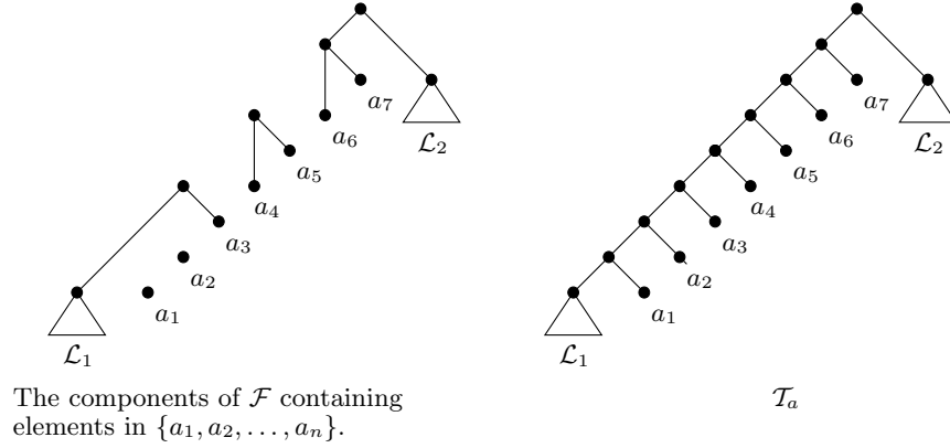
FIGURE 7. Joining the components of \mathcal{F} containing elements in \{a_1, a_2, \dots, a_n\} to form a new component \mathcal{T}_a in \mathcal{F}' .
