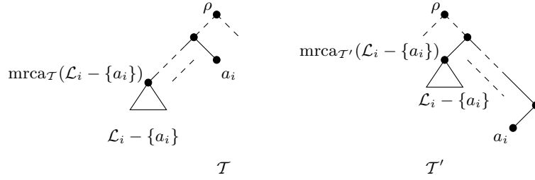
FIGURE 6. Under the assumption that this configuration appears in \mathcal{F} , then the rest of the members of \{a_1, a_2, \dots, a_n\} - \{a_i\} must label isolated vertices in \mathcal{F} .
