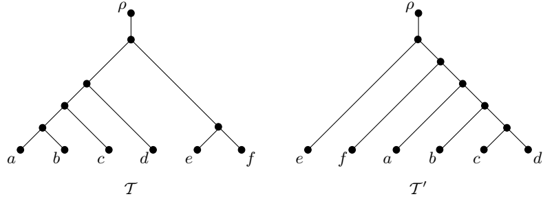
FIGURE 2. Two rooted binary phylogenetic trees with their roots labelled.
