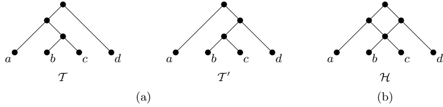
FIGURE 1. (a) Two rooted binary phylogenetic trees \mathcal{T} and \mathcal{T}' and (b) a hybridization network \mathcal{H} that displays them.
