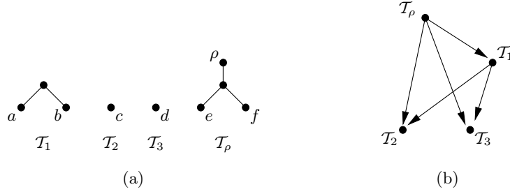
FIGURE 3. (a) A maximum-acyclic-agreement forest \mathcal{F} for \mathcal{T} and \mathcal{T}' in Fig. 2 and (b) the graph G_{\mathcal{F}} .
