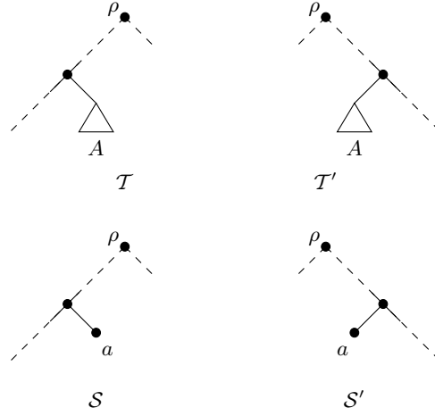
FIGURE 4. Two weighted phylogenetic trees reduced under Rule 1, where \mathcal{S} and \mathcal{S}' are the resulting trees.
