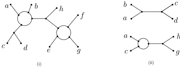
Fig. 1 (i) A level-1 phylogenetic network with leaf-set X = \{a, b, \dots, h\} . (ii) Top: a quartet tree with leaf-set \{a, b, c, d\} , also denoted by ab|cd . Bottom: a quarnet with leaf-set \{a, c, h, g\} . Both the quartet tree and quarnet are displayed by the level-1 network in (i).
