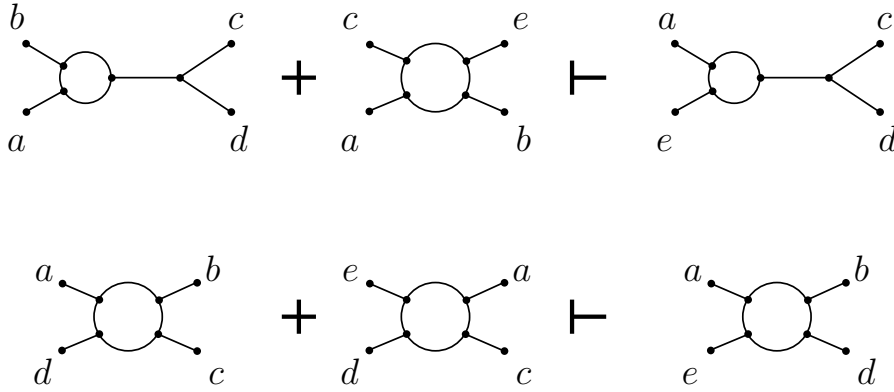
Fig. 5 An illustration of the (CL2) and (CL3) inference rules. Top: The first part of the (CL2) inference rule with * = \ominus . Bottom: the (CL3) inference rule.
