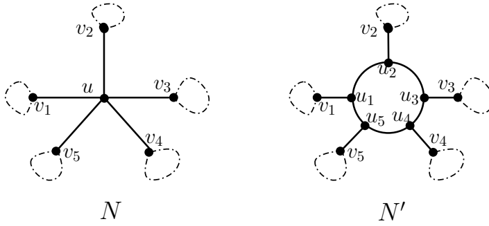
Fig. 2 Example of blow-up operations: N' is obtained from N by a blow-up operation on u .
