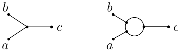
Fig. 3 The two types of three-leaved networks: tree type (left) and cycle type (right).
