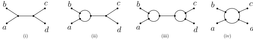
Fig. 4 Four types of qnets on X = \{a, b, c, d\} : (i) a Type I qnet a \ominus b|c \ominus d ; (ii) a Type II qnet a \oplus b|c \ominus d ; (iii) a Type III qnet a \oplus b|c \oplus d ; (iv) a Type IV qnet a \oplus b \oplus c \oplus d . Type IV is of cycle type.
