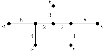
FIGURE 4. An phylogenetic tree with edge lengths. Here \{a, c, d, e\} is the unique subset of size 4 that maximizes M(\{a, c, d, e\}) = 12 , but it does not contain \{a, b, c\} , the unique subset of size 3 that maximizes M(\{a, b, c\}) = 13 .
