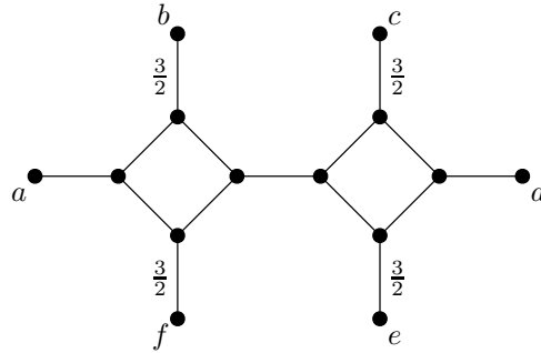
FIGURE 5. A split network [14] corresponding to a circular split system. Apart from the edges with weight \frac{3}{2} , all edges have weight 1. Here \{b, c, e, f\} is a subset of size 4 that maximizes PD(\{b, c, e, f\}) = 11 , but it does not contain \{a, d\} , the unique set of size 2 that maximizes PD(\{a, d\}) = 7 .
