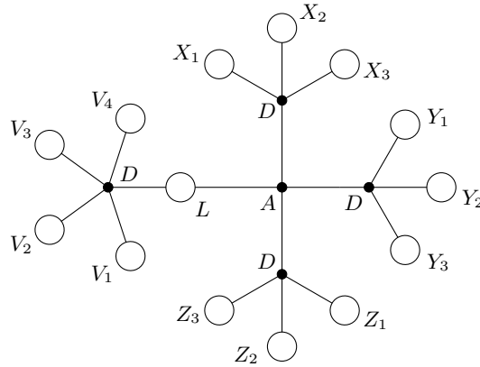
FIGURE 3. The 3-tree T .
