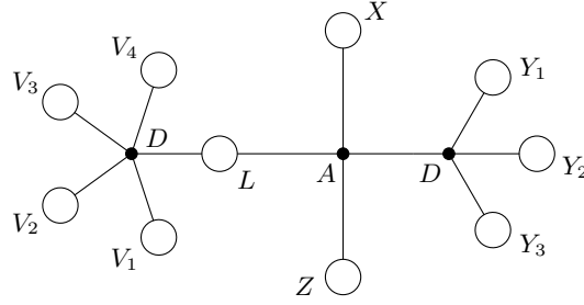
FIGURE 4. The path realization T_1 .
