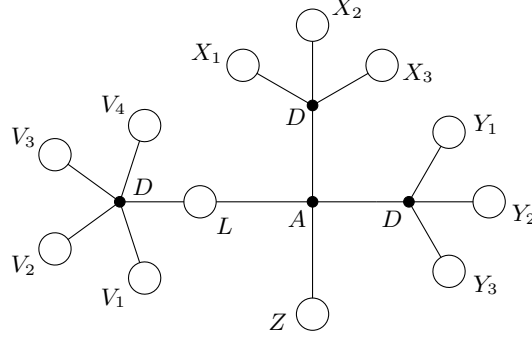
FIGURE 5. The \pi -labelled tree T_2 .
