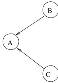
Fig. 1. Directed acyclic graph.
