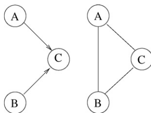
Fig. 2. Moralization of a directed acyclic graph.
