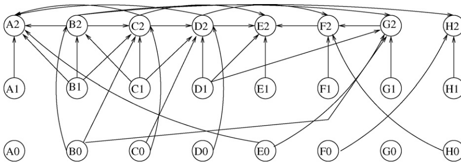
Fig. 5. Alternative model.
