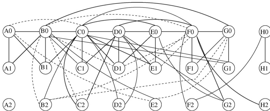
Fig. 3. Conditional independence graph.
