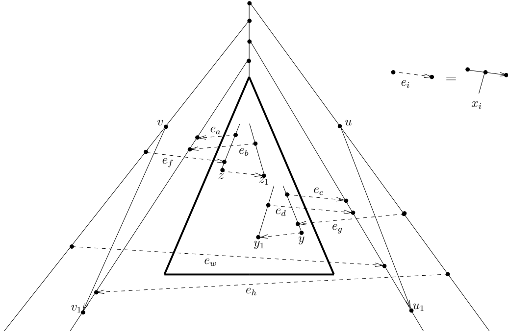
Fig. 6 The HGT network \mathcal{N} constructed from \mathcal{N}' in the proof of Theorem 35. The part of the network enclosed by the solid triangle is the same as that shown in Figure 5 except that vertices u , u_1 , v , and v_1 have been renamed as y , y_1 , z , and z_1 , respectively. Each dashed line e_i with i \in \{a, b, c, d, f, g, h, w\} represents a 2-arc directed path (with the middle vertex omitted) and the attachment of a new taxa x_i (also omitted) adjoined to the middle vertex on the path, see top right of the figure. This means that the endpoint of each dashed line corresponds to a non-critical HGT vertex.
