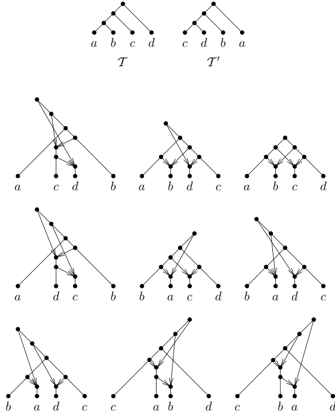
Fig. 8 Two rooted binary phylogenetic X -trees \mathcal{T} and \mathcal{T}' , and all nine hybridization networks on X displaying both trees with two hybridization vertices. None of the hybridization networks is temporal.
