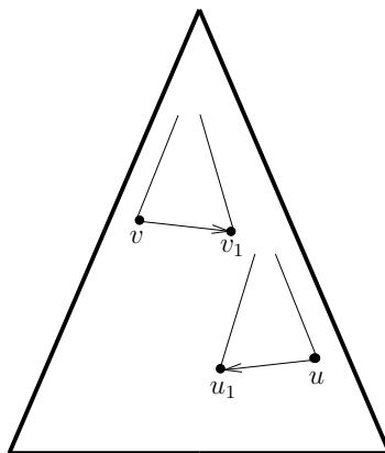
Fig. 5 The bold triangle represents the HGT network \mathcal{N}' in the proof of Theorem 35. Only the vertices u, u_1, v, and v_1 are drawn explicitly as we need them to obtain \mathcal{N} from \mathcal{N}' (see Figure 6). Note that u is not an ancestor of v_1 , however, v is an ancestor of u_1 if (v, u) is an arc in G' .
