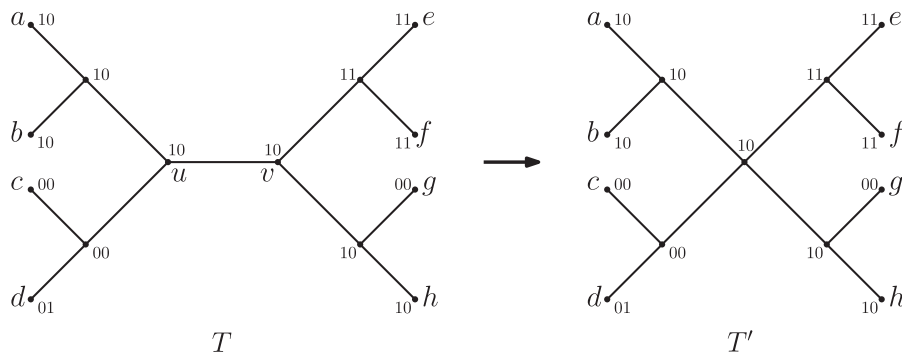
Fig. 1. T' = T \setminus e ; removing an edge with no change for any character does not change the parsimony score.
