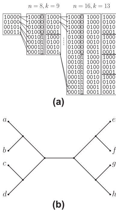
Fig. 2. The balanced tree construction based on Chai and Housworth (2011). (a) The number of taxa can be doubled by repeating each taxon and then adding four new characters at the end of each sequence, repeating the pattern 1000, 0100, 0010, 0001. (b) The tree topology for eight taxa, where a, b, \dots, h are labeled with the 1st, 2nd, \dots , 8th row in column two of (a). The interior nodes can be labeled such that each edge has a change for exactly one character, and the parsimony score therefore equals the number of edges.
