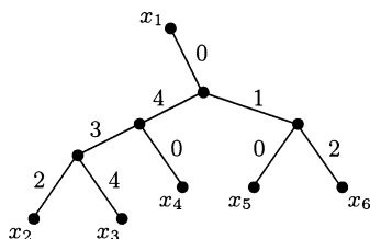
FIG. 3. A \mathbb{Z}_5 -edge coloring.
