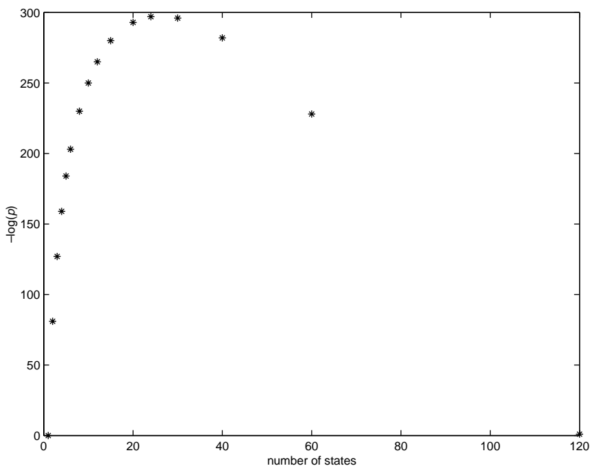
FIG. 2. Distribution of trivalent phylogenetic trees on 120 leaves by the number of character states.
