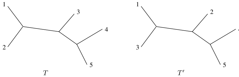
Fig. 1. Two binary phylogenetic X-trees for X = \{1, 2, 3, 4, 5\} . If we take Y = \{1, 2, 3, 4\} then T|Y = 12|34 and T'|Y = 13|24 .
