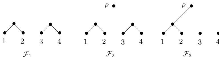
FIGURE 3. A maximum-agreement forest \mathcal{F}_1 for \mathcal{T} and \mathcal{T}' of Fig. 2 under the definition in [8], and two maximum-agreement forests \mathcal{F}_2 and \mathcal{F}_3 for \mathcal{T} and \mathcal{T}' under our definition.
