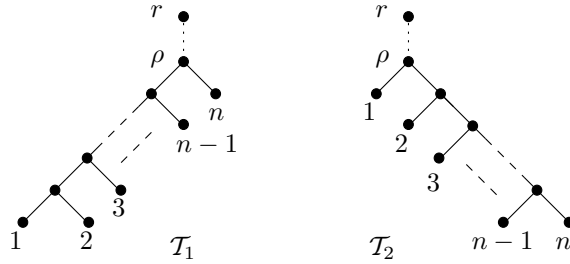
FIGURE 4. Two rooted binary phylogenetic trees.
