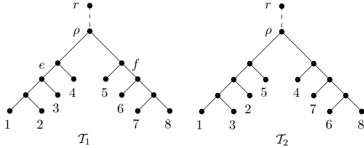
FIGURE 7. The distances between \mathcal{T}_1 and \mathcal{T}_2 differ for each metric.
