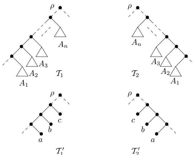
FIGURE 6. Two rooted binary phylogenetic trees reduced under Rule 2*.
