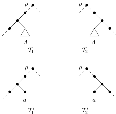
FIGURE 5. Two rooted binary phylogenetic trees reduced under Rule 1.
