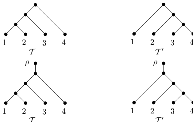
FIGURE 2. Two rooted binary phylogenetic trees \mathcal{T} and \mathcal{T}' , pictured without (above) and with (below) their roots labelled.
