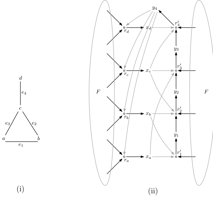
Figure 6: (i) A graph G and (ii) the associated CRS \mathcal{Q}_G , consisting of 8 reactions that form an RAF, and with the super-catalyst ( y_4 ) at the top. The two smallest sub-RAF's of this system are formed by adding either r_a and r_c or r_b and r_c to the four reactions r'_1, \dots, r'_4 , and these two choice correspond to the two smallest vertex covers of G , namely \{a, c\} and \{b, c\} .
